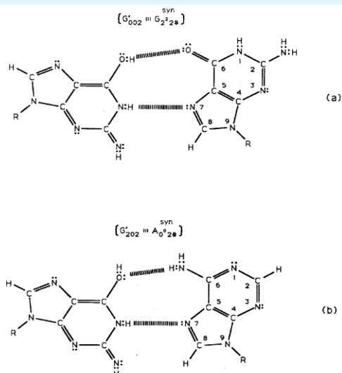
Figure 6: Complementary transversion mispairs created by enzyme-proton entanglement executing a “truncated” Grover’s quantum search. Complementary mispairs between (a) enol-imine G'002 (Figure 5b) and syn -guanine ( syn - G_{2'2\#} ) and (b) enol-imine G'202 (Figure 5c) and syn -adenine ( syn - A_{0'2\#} ). The # symbol indicates the position is occupied by ordinary hydrogen unsuitable for hydrogen bonding.
