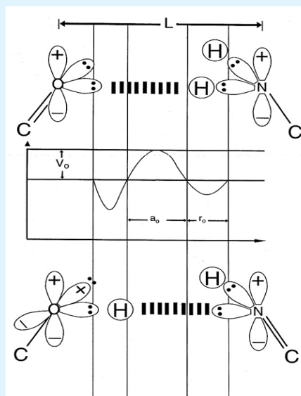
Figure 1: Schematic of “metastable” keto-amino and “ground state” enol-imine hydrogen bonds.
