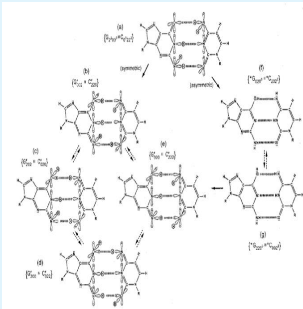
Figure 3: Distribution of entangled proton qubit states at a G'-C' (symmetric) or *G'-*C (asymmetric) superposition site. Symmetric, asymmetric and second asymmetric (unlabeled) channels ( \rightarrow ) by which metastable keto-amino G-C protons populate enol and imine entangled proton qubit states. Dashed arrows identify pathways for quantum oscillation of enol and imine proton qubits. Approximate electronic structures for hydrogen bond end groups and corresponding proton positions are shown for the metastable keto-amino duplex (a) and for enol and imine entangled proton qubit states, G'-C' (b-e). Electron lone-pairs are represented by double dots, :, and a proton by a circled H. Proton states are specified by a compact notation, using letters G, C, A, T for DNA bases with 2's and 0's identifying electron lone-pairs and protons, respectively, donated to the hydrogen bond by - from left to right - the 6-carbon side chain, the ring nitrogen and the 2-carbon side chain. Superscripts identify the component at the outside position (in major and minor grooves) as either an amino group proton, designated by 0^0 , or a keto group electron lone-pair, indicated by 2^2 . Superscripts are suppressed for enol and imine groups.)
