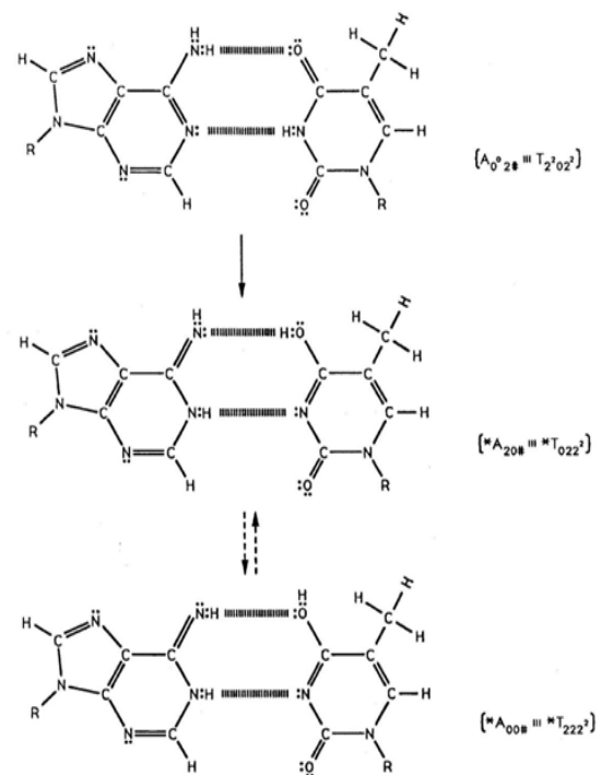
Figure 4: Pathway for metastable keto-amino A-T protons to populate enol and imine proton qubit states. Dashed arrows indicate proton oscillatory pathway for enol and imine proton qubit *A-*T states. Notation is given in Figure 3 legend. The # symbol indicates the position is occupied by ordinary hydrogen unsuitable for hydrogen bonding.
